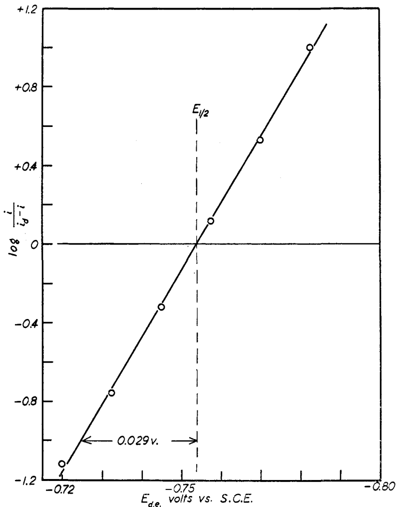
FIG. 2. Test of the equation of the wave of the biplumbite ion. Experimental points from figure 1.
