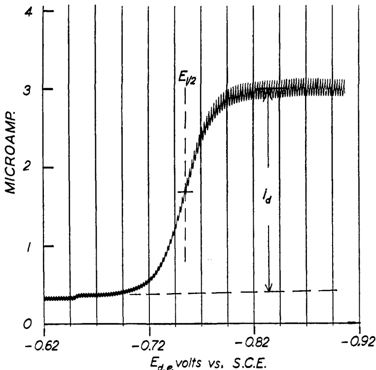
FIG. 1. Polarogram of 5 \times 10^{-4} M lead nitrate in 1.09 N sodium hydroxide at 25°C.
